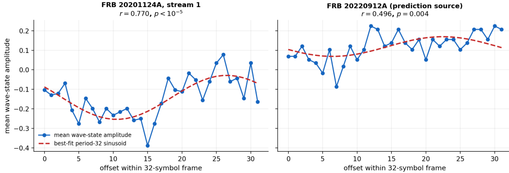
Figure 3: Mean wave-state amplitude across the 32 offsets, with best-fit sinusoid: one complete wavelength per frame. Left: FRB 20201124A, stream 1 ( r = 0.770 ). Right: FRB 20220912A under the same pipeline ( r = 0.496 , p = 0.004 ); Section 6 gives this source’s prediction history.
