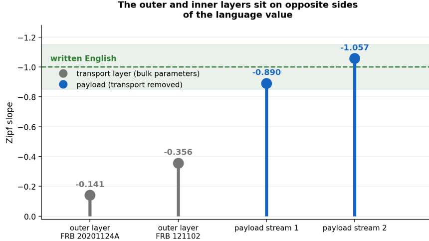
Figure 7: The central result. The outer transport layer and the inner content layer sit on opposite sides of the written-English value; FRB 121102’s outer layer, measured identically, confirms the transport side independently. All four values are printed by the analysis script.
