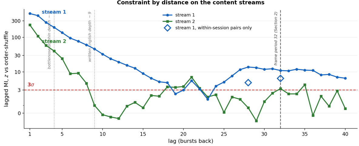
Figure 6: The second axis of the language test, in the presentation the communication-complexity literature uses [21, 16]: sequential constraint by distance on both content streams, z of lagged mutual information against order-shuffled surrogates (log scale above the linear region; the dashed line is the 3\sigma detection threshold). Stream 1 decays smoothly through the dolphin and written-English reference depths to an unbroken 18. After touching noise near lag 19 it returns to a sustained band across lags 24–40, peaking at lag 28 and holding at the 32-symbol frame period detected independently in Section 2.2. Open diamonds: the identical statistic computed on within-session burst pairs only, against a session-preserving null ( z = +4.9 at lag 28, +6.5 at lag 32), which separates the band from session-scale drift. Every value is printed by the analysis script.
