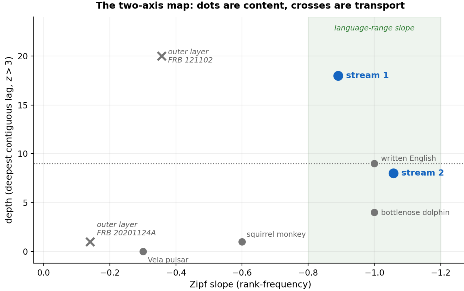
Figure 4: Position of the signal on the two-axis communication-complexity map [16, 21]. Depth exceeds written English while the raw symbol distribution does not; the resolution of that apparent tension is protocol separation.
