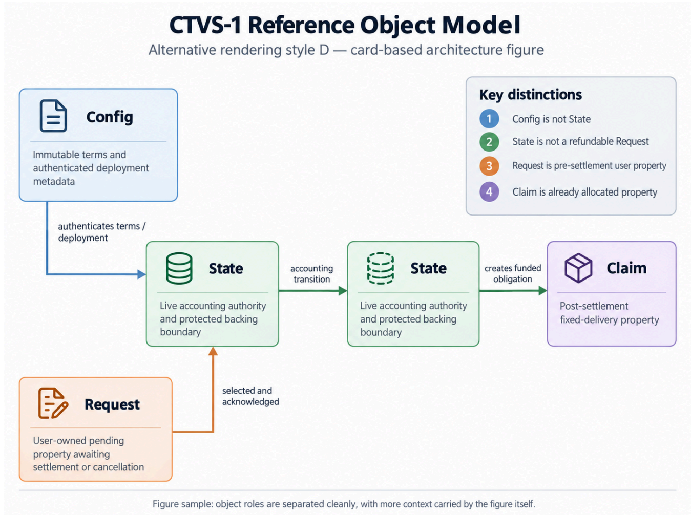
Figure 2: Authenticated reference objects and the economic boundary. Config, State, Request, and Claim have distinct authentication, ownership, and spending roles. A request-shaped datum cannot route genuine State custody through a refund branch.
