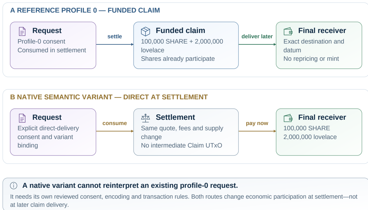
Figure 5: Two settlement dispositions, one economic cutover. Profile 0 creates a funded Claim for later delivery; the native direct-delivery variant pays the final receiver inside settlement. One request interpretation cannot silently switch between them.
