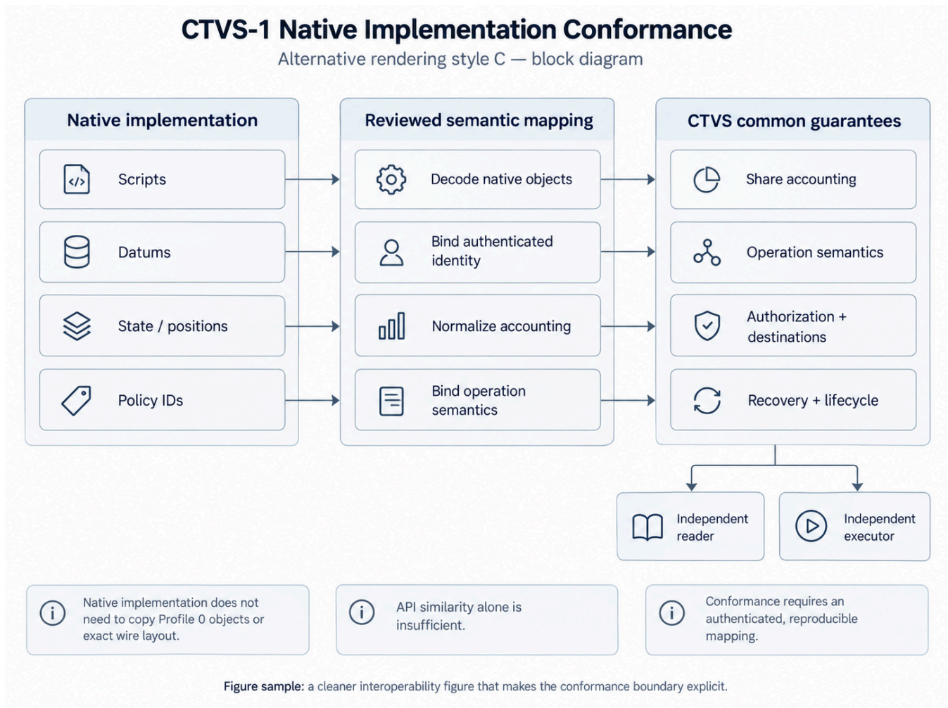
Figure 1: One standard boundary, two implementation paths. A native protocol may retain its own scripts and datums, but execution conformance requires a reviewed mapping to the same authenticated economic guarantees. Matching JSON or labels alone is not sufficient.
