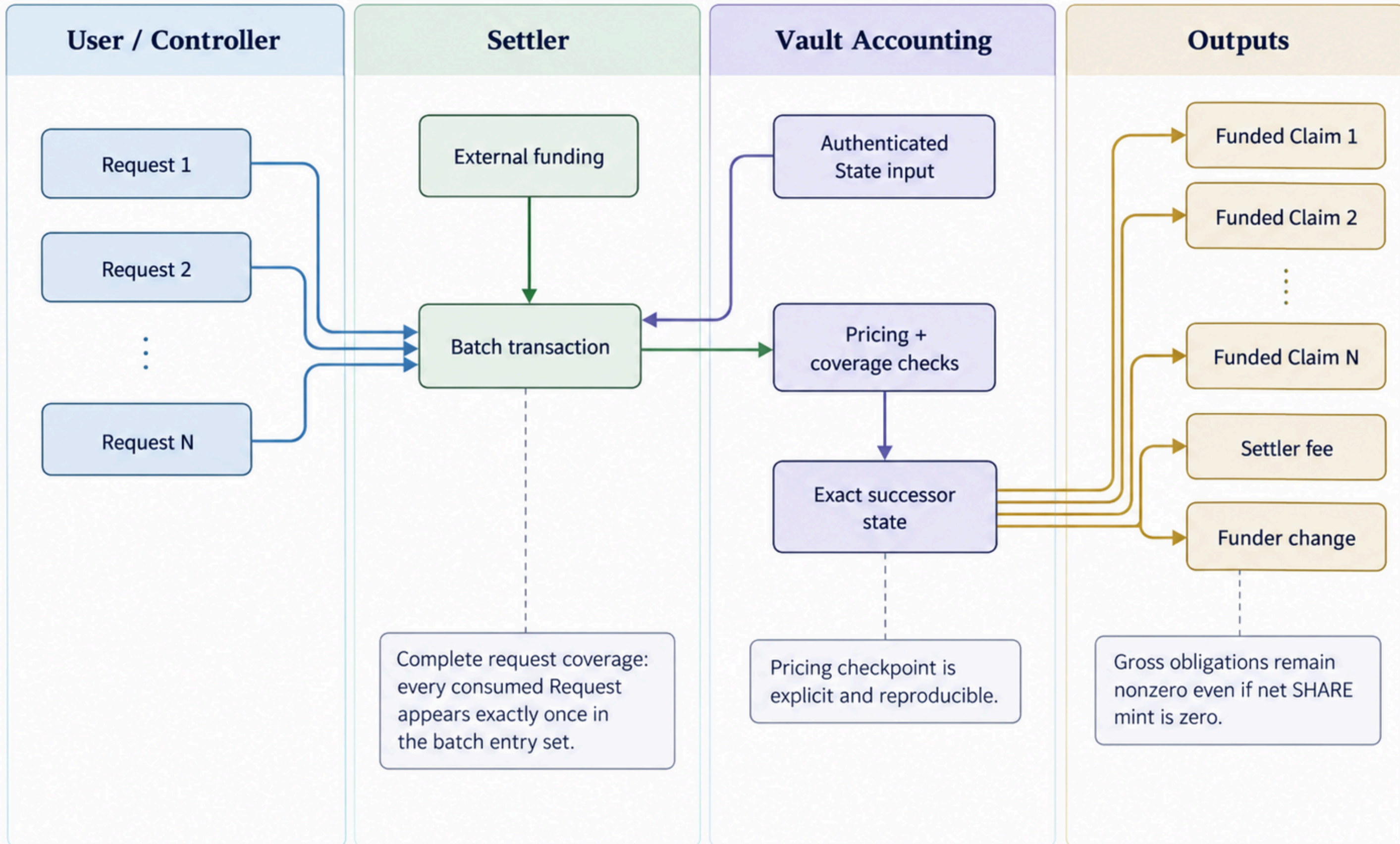
Figure sample: swimlane rendering emphasizes actors, accounting checkpoints, and output obligations.
