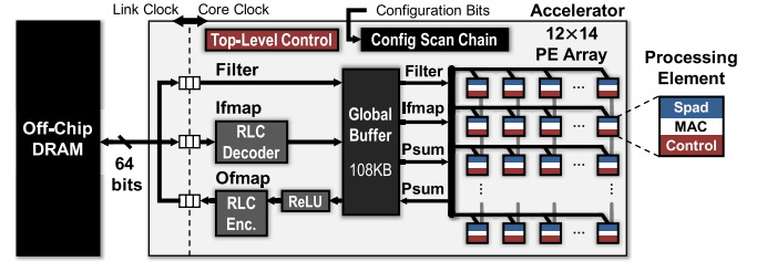
Fig. 2. Eyeriss system architecture.
