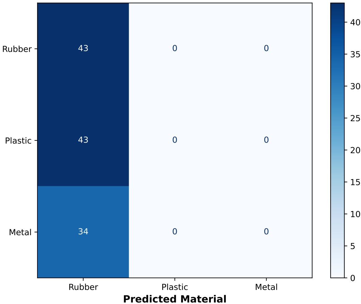
Tactile Transformer Confusion Matrix
