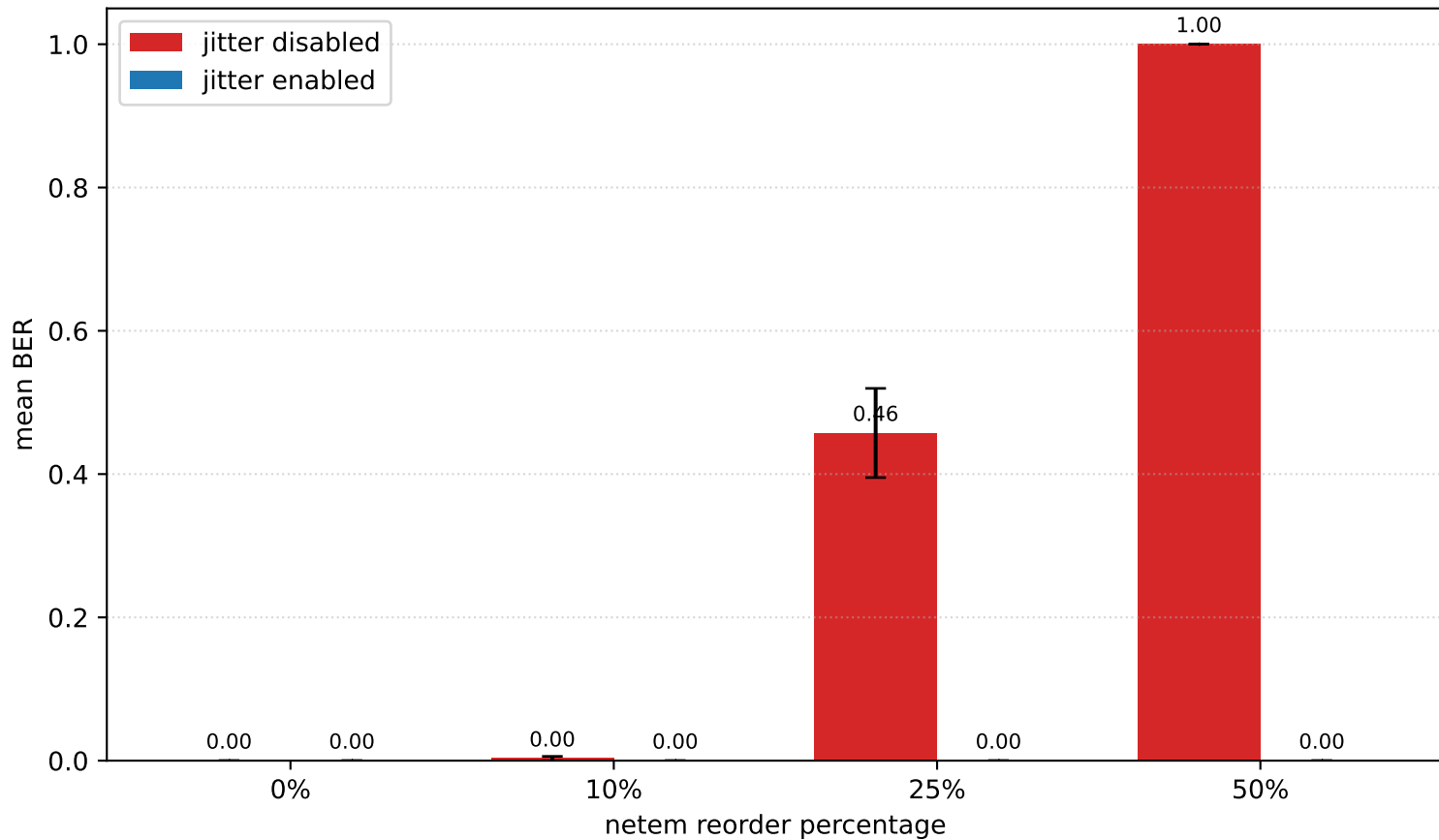
Jitter buffer ablation: byte error rate
