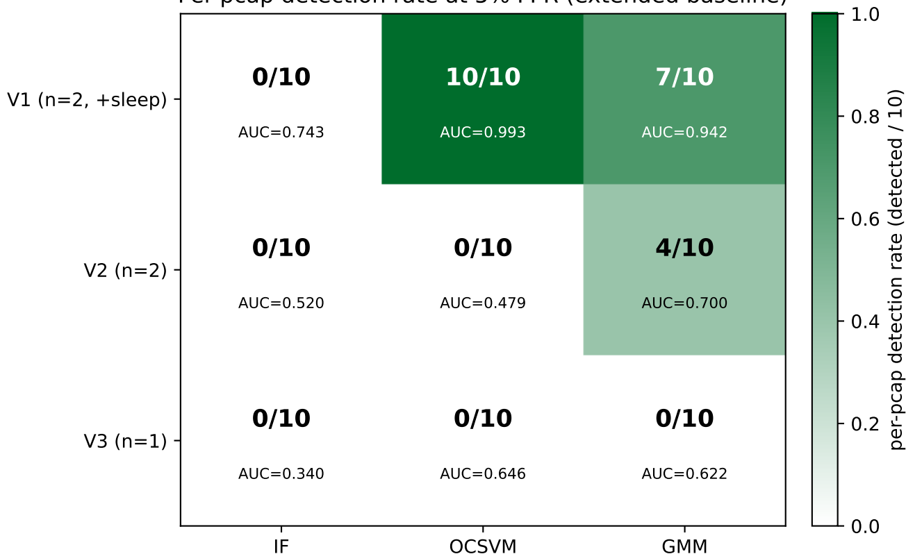
Per-pcap detection rate at 5% FPR (extended baseline)
