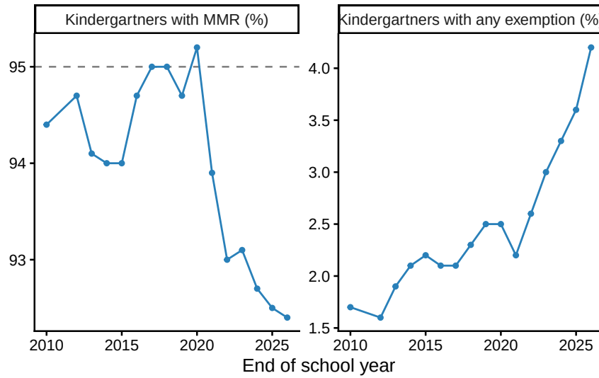
Figure 4.5: MMR vaccination coverage (left) and exemption rate (right) among US kindergartners, school years 2009–10 to 2025–26. The dashed line marks 95% coverage. Data: CDC SchoolVaxView (state-reported); the 2010–11 school year was not reported. Note that coverage is measured at school entry.
