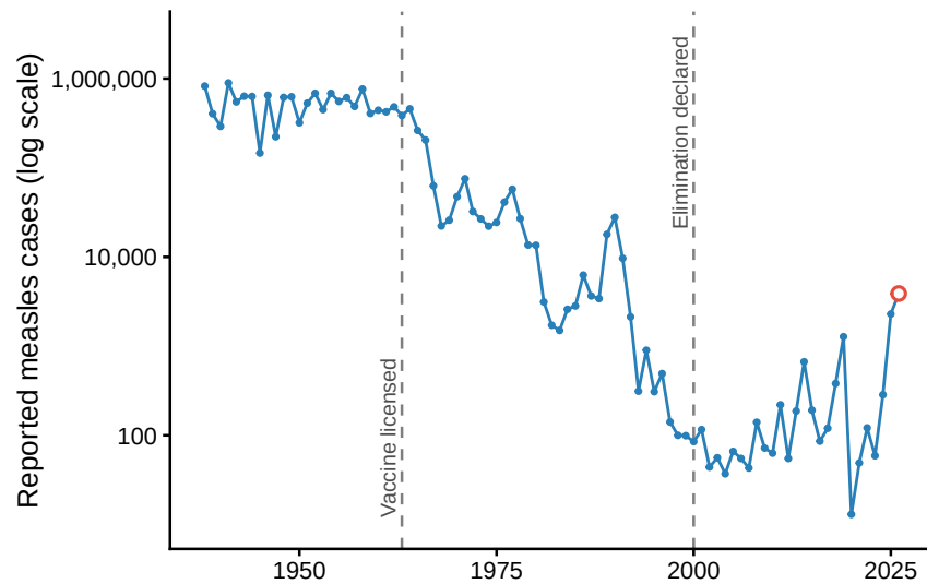
Figure 4.4: Reported measles cases in the US, 1938–2026 (log scale). Data from the CDC and earlier public health reports, compiled by Our World in Data. Dashed lines mark the licensure of the first measles vaccine (1963) and the declaration that measles was eliminated from the US (2000). The 2026 count (open circle) is incomplete: it covers cases through October 1.
