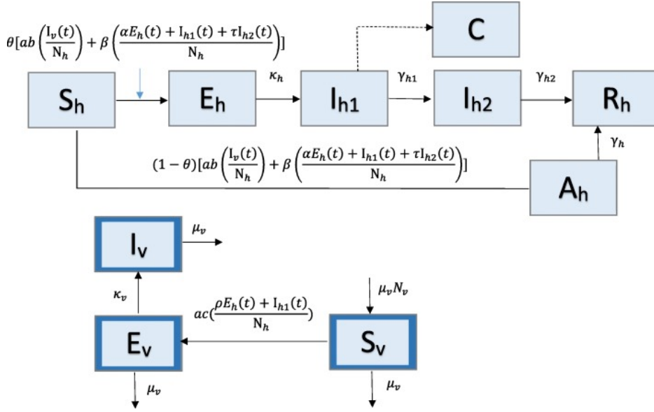
Figure 4.9: Compartmental diagram for the Zika virus transmission model of Roosa and Chowell (2019). The human population (top) is divided into six classes; the mosquito (vector) population (dark blue outline) into three. Arrows are labelled with the rates governing transitions between compartments.
