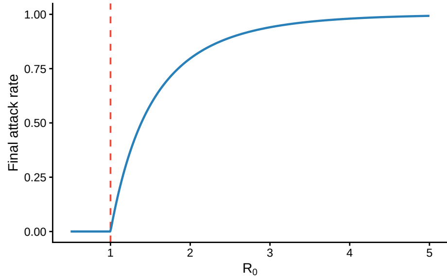
Figure 4.3: Final attack rate 1 - S(\infty) as a function of R_0 , obtained by solving Equation 4.1 numerically. Below the epidemic threshold R_0 = 1 (red dashed line) the infection always dies out; above it a non-zero fraction of the population is infected. For R_0 = 2 , approximately 80% of a fully susceptible population is eventually infected before the epidemic ends.
