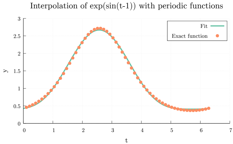
Figure 6: Least square fit of \exp(\sin(t-1)) with Fourier periodic functions
