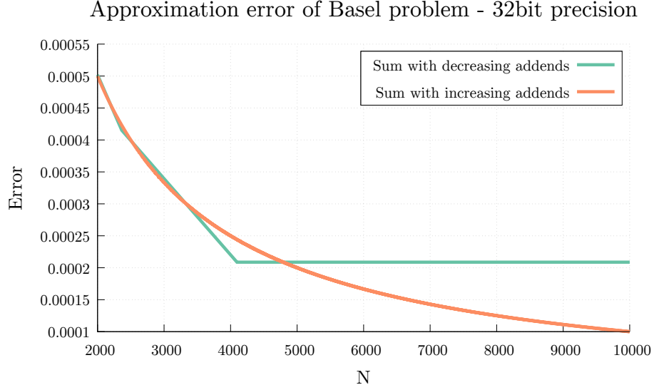
Figure 2: Approximation error when computing \pi^2/6 with the Basel problem truncated series \sum_0^N \frac{1}{n^2} , with single precision floating variables. Here N is the number of terms used when calculating the series.
