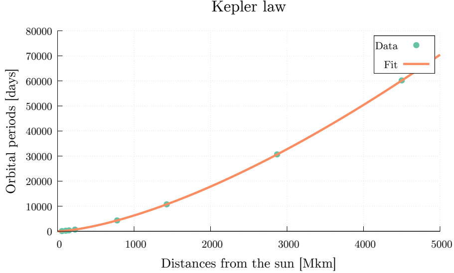
Figure 4: Orbital peirods vs distances from the Sun of the planets.
