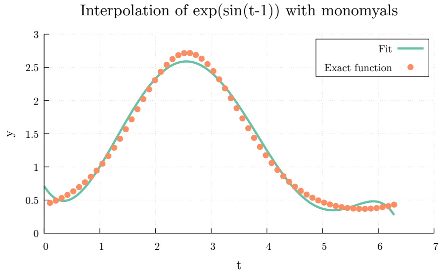
Figure 5: Least square fit of \exp(\sin(t-1)) with 6th degree polynomial
