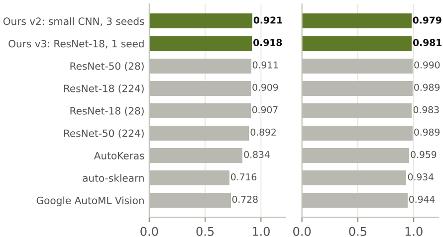
Test accuracy
