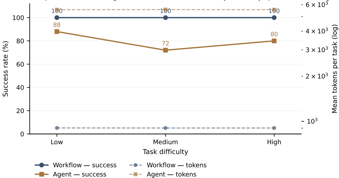
Archetype D — Compliance Decisioning — success and token cost by difficulty (pooled over all grid runs)
