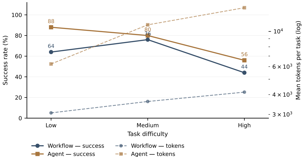
Archetype G — Strategic Planning — success and token cost by difficulty (pooled over all grid runs)
