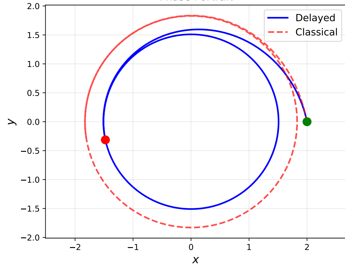
Phase Portrait
