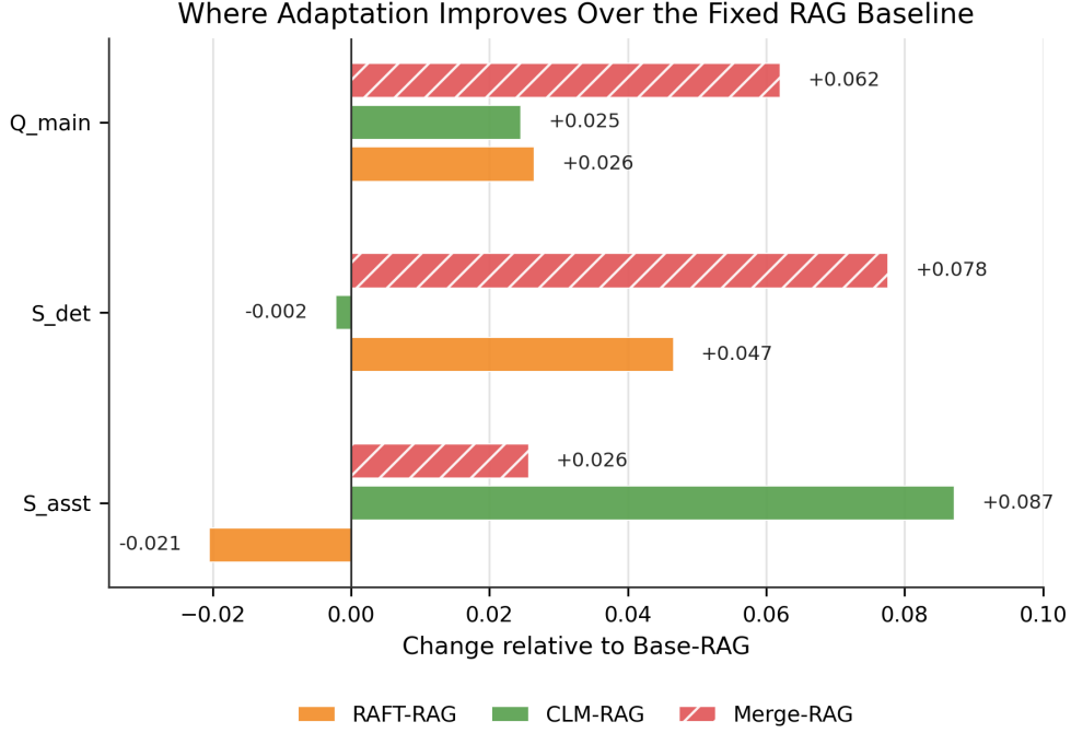
Figure 2: Improvement over Base-RAG. Grouped bars show the observed Delta-Q_main, Delta-S_det, and Delta-S_asst point estimates for RAFT-RAG, CLM-RAG, and Merge-RAG. Paired intervals for the predefined headline Q_main contrasts are reported in Table 3.
