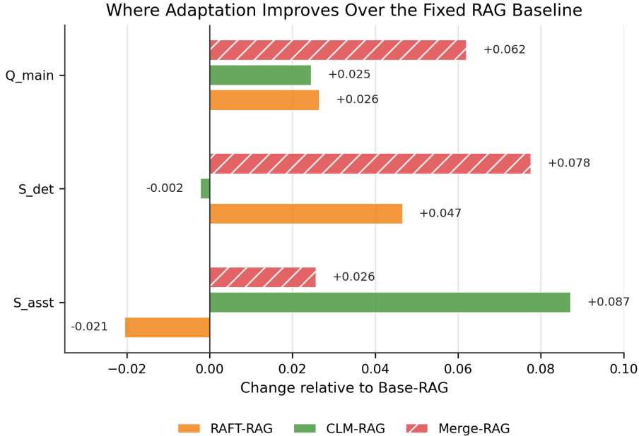
Figure 2: Improvement over Base-RAG. Grouped bars show the observed Delta- Q\_main , Delta- S\_det , and Delta- S\_asst point estimates for RAFT-RAG, CLM-RAG, and Merge-RAG. Paired intervals for the predefined headline Q\_main contrasts are reported in Table 3.
