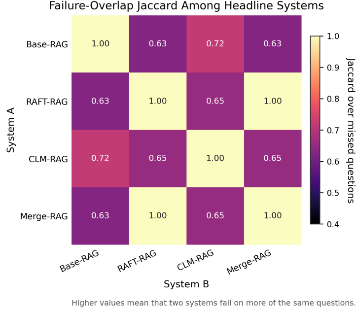
Figure B.1: Failure-overlap Jaccard among headline systems. Higher values indicate that two systems fail on more of the same evaluation questions.
