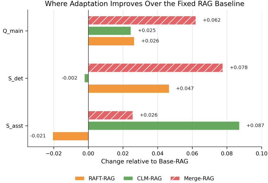
Figure 2: Improvement over Base-RAG. Grouped bars show Delta- Q_{\text{main}} , Delta- S_{\text{det}} , and Delta- S_{\text{asst}} for RAFT-RAG, CLM-RAG, and Merge-RAG. RAFT raises S_{\text{det}} , CLM raises S_{\text{asst}} , and the merge raises both.
