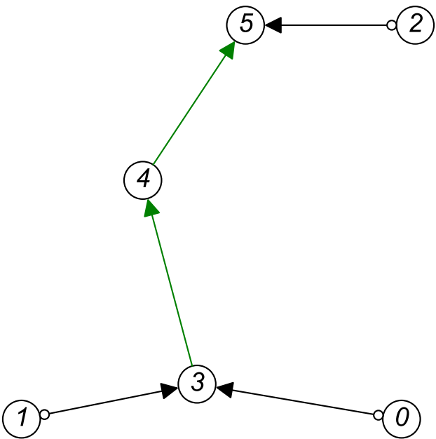
Data-Level PAG Fold 5
