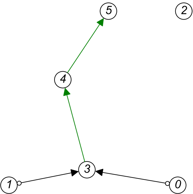
Data-Level PAG Fold 4
