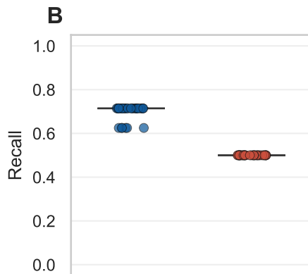
Benchmark-to-Model Detection of Output Intervention Effects
