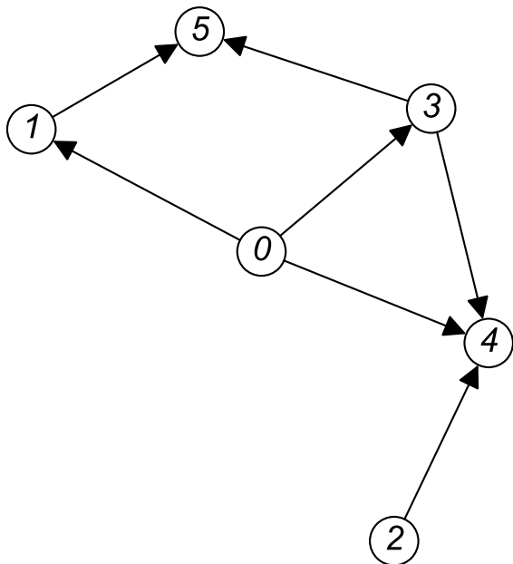
Ground Truth DAG (Linear SEM)
