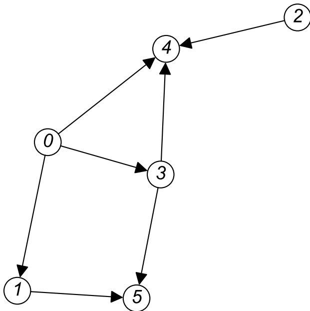
Ground Truth DAG (Linear SEM)
