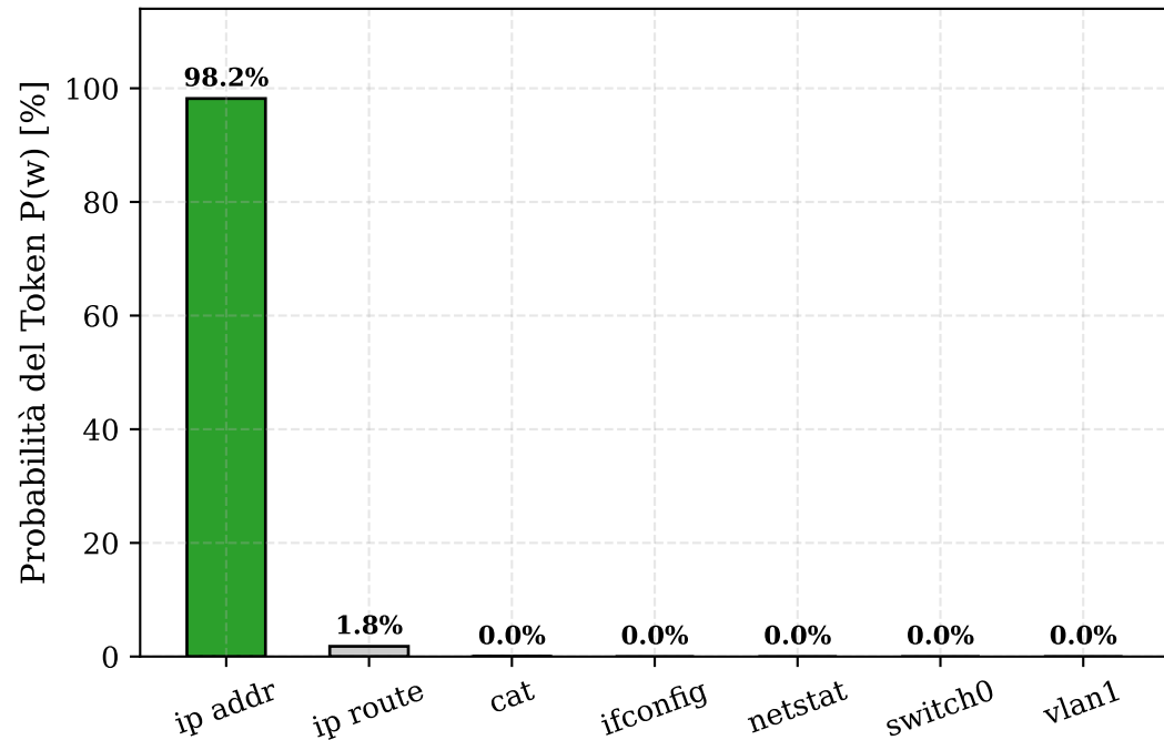
Profilo C (T = 0.1, Top-p = 0.5) — Quasi-Greedy
