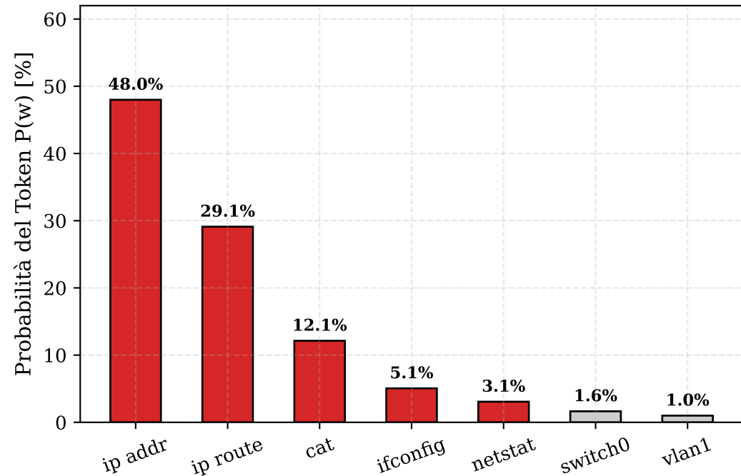
Profilo A (T = 0.8, Top-p = 0.9) — Alta Entropia
