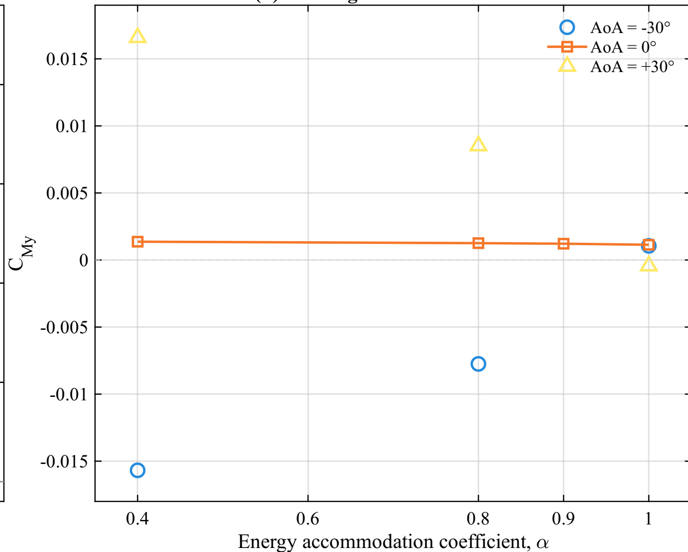
(b) Pitching-moment coefficient
