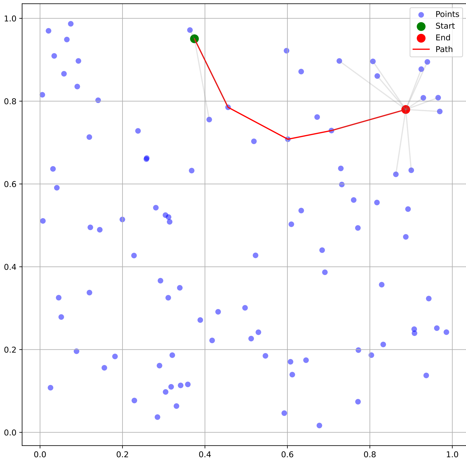
Shortest Path
