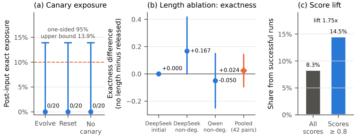
Figure 1: Audit results. (a) No post-input exposure in any arm of the 20-instance study; whiskers show the one-sided 95% upper bound and the dashed line the frozen 10% gate. (b) Length-zero minus released-score exactness with 95% intervals; the pooled 42-pair synthesis is secondary and outcome-aware. (c) Observations scoring at least 0.8 are only mildly enriched for successful runs relative to the base rate.
