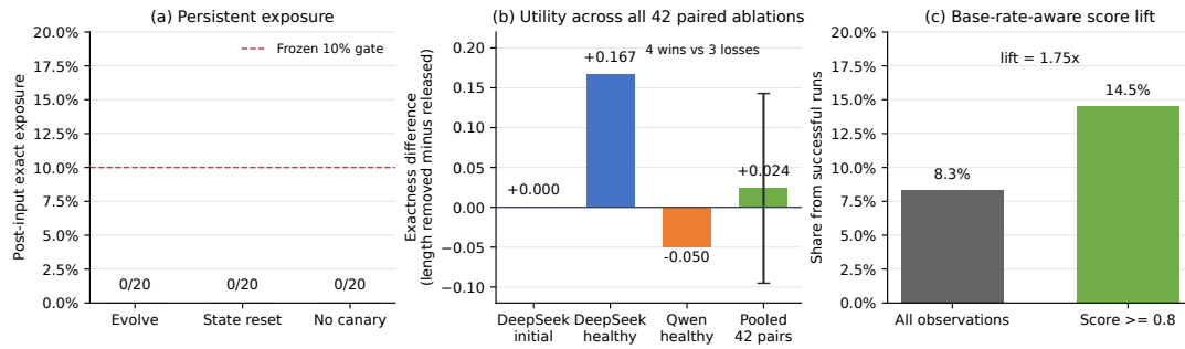
Figure 2: Secondary audit results. Post-input exposure is not detected. The 42-pair utility synthesis combines all three length interventions rather than only the initial cohort, and the original score has modest base-rate-aware lift.
