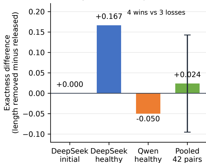
(b) Utility across all 42 paired ablations
