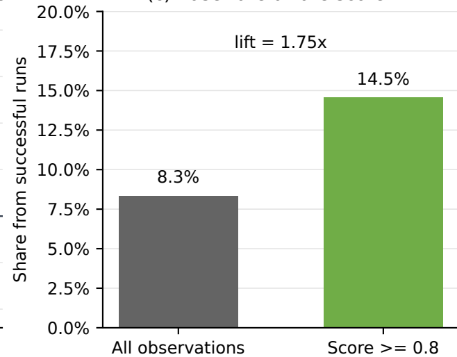
(c) Base-rate-aware score lift
