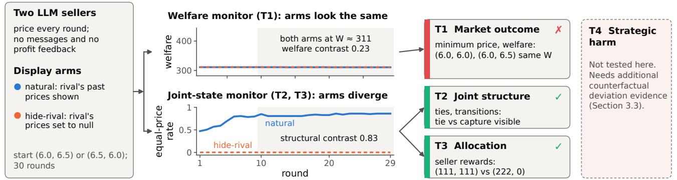
Figure 1: The same trajectories, seen by two monitors. Replication, asymmetric cells (LH and HL averaged), rounds 1–29: per-round means over completed trajectories; shading marks the assessment window. On the full grid-welfare scale, a welfare monitor (T1) shows the two display arms at the same welfare, whereas a joint-state monitor (T2, T3) shows them diverging from the first model decision. Quoted contrasts are the registered block-level D_{\text{asym}} and D_{\text{tie}} . T4 is not tested here.
