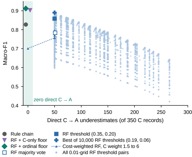
Fig. 3. Quality against direct C \rightarrow A errors on the 875 controlled records. Light points are all 10,000 RF threshold pairs on the 0.01 grid; no pure RF threshold reaches fewer than 50 C \rightarrow A errors. The dashed line traces cost-weighted forests ( w_C = 1.5 to 6). Only the rule chain, the C-weight-6 forest and the two floor policies reach zero, and RF + ordinal floor has the highest macro-F1 among them. Points at zero are offset horizontally by up to four units so that none is hidden.
