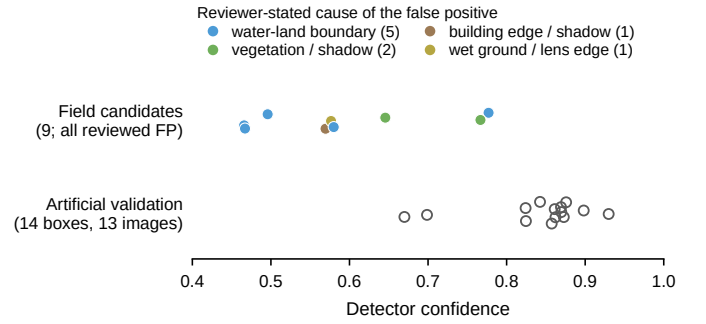
Fig. 5. Detector confidence of the nine reviewed field candidates, coloured by the reviewer-stated cause of the false positive, and of the 14 boxes on artificial-piping images (no review status or missed-detection record). Vertical position within a row is jitter for visibility.
