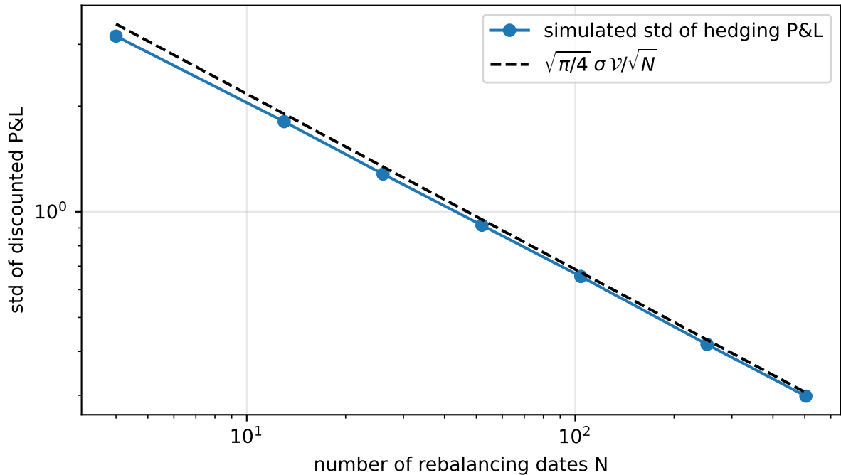
Hedging error vs rebalancing frequency (slope -0.489)
