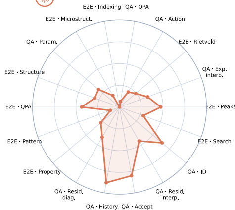
Claude Haiku 4.5
