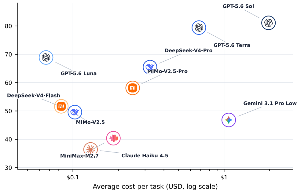
d Cost-effectiveness by price
