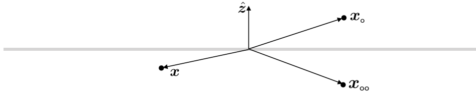
FIGURE 8.7: Illustrating the method of images for the half-plane, in which the Green's function is singular at the source point, \mathbf{x}_o = \hat{\mathbf{x}} x_o + \hat{\mathbf{y}} y_o + \hat{\mathbf{z}} z_o , located in the upper half-plane ( z_o > 0 ). The image source point at \mathbf{x}_{oo} = \hat{\mathbf{x}} x_o + \hat{\mathbf{y}} y_o - \hat{\mathbf{z}} z_o is located in the lower half-plane. For the Dirichlet problem the sources have the opposite sign, thus ensuring that the Green's function vanishes for field points, \mathbf{x} , evaluated on the boundary at z = 0 . For the Neumann problem, both sources have the same sign, which renders \partial_z G = 0 for field points on the boundary at z = 0 .
