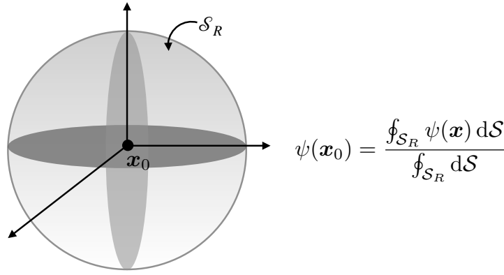
FIGURE 8.1: The value of a harmonic function at a point \mathbf{x}_0 equals to the area average of the function over a sphere of arbitrary radius (so long as \nabla^2\psi = 0 inside the sphere) centered at \mathbf{x}_0 . We here illustrate this property for 3-dimensions, with this property holding for arbitrary space dimensions, n \geq 1 . The mean value property for harmonic functions implies that there can be no extrema of \psi within the domain, for if there was an extrema then we could no longer guarantee that the average value around all surrounding spheres equals to the value at the extrema. Hence, extrema of harmonic functions live on the domain boundary.
