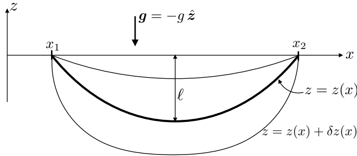
FIGURE 7.5: A massive string or cable is supported at its two ends at a vertical position z_1 = z(x_1) = z_2 = z(x_2) . The string is placed in a vertically directed gravitational field with acceleration, \mathbf{g} = -g\hat{\mathbf{z}} , where g is the constant gravitational acceleration. Variational methods determine the shape of the string as given by the hyperbolic cosine in equation (7.106), which is known as a catenary . This is the ideal shape taken by stationary power lines, spider webs, clothes lines, and chains, for example.
