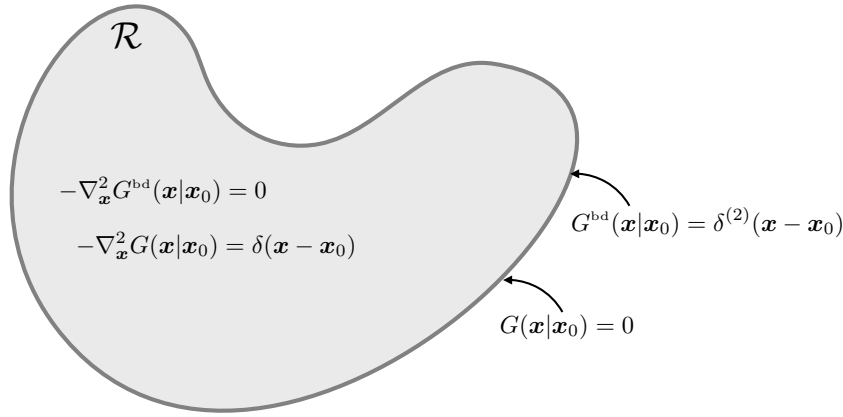
FIGURE 8.4: Decomposing the Green's function solution (8.146) for a Poisson boundary value problem with Dirichlet boundary conditions. The decomposition is written in terms of an interior Green's function, G(\mathbf{x}|\mathbf{x}_0) , that satisfies equation (8.128) with both the field point, \mathbf{x} , and Dirac source point, \mathbf{x}_0 , within the domain, \mathbf{x}, \mathbf{x}_0 \in \mathcal{R} . The second piece of the solution arises from the boundary Green's function, G^{bd}(\mathbf{x}|\mathbf{x}_0) , with the source point on the boundary, \mathbf{x}_0 \in \partial\mathcal{R} . The boundary Green's function satisfies the boundary value problem (8.157a)-(8.157b), in which G^{bd} is harmonic for \mathbf{x} \in \mathcal{R} , and it is a Dirac delta when sampled on the boundary, \mathbf{x} \in \partial\mathcal{R} .
