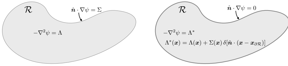
FIGURE 8.5: Use of Neumann boundary conditions for the Poisson boundary value problem allows for two equivalent formulations of how the boundary data is handled. The first, shown in the left, considers the Poisson equation -\nabla^2\psi = \Lambda satisfied within the domain, \mathbf{x} \in \mathcal{R} , along with boundary data along \mathbf{x} \in \partial\mathcal{R} , where \hat{\mathbf{n}} \cdot \nabla\psi = \Sigma . The second formulation, shown on the right, absorbs the boundary data into the domain source via a Dirac delta sheet that is placed infinitesimally close, on the inside, of the boundary. In this approach the Poisson equation has a modified source, \Lambda^*(\mathbf{x}) = \Lambda(\mathbf{x}) + \Sigma(\mathbf{x})\delta[\hat{\mathbf{n}} \cdot (\mathbf{x} - \mathbf{x}_{\partial\mathcal{R}})] , and the Neumann boundary condition is now homogeneous, \hat{\mathbf{n}} \cdot \nabla\psi = 0 . The delta sheet is here depicted by the slightly thicker line placed around the boundary.
