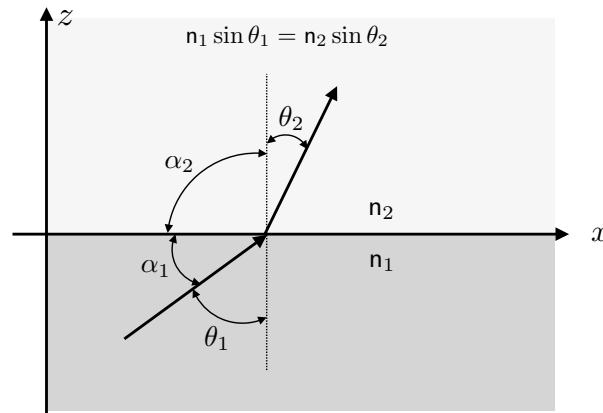
FIGURE 7.6: Illustrating Snell's law , n_1 \sin \theta_1 = n_2 \sin \theta_2 , where n > 0 is the index of refraction for the media, assumed here to be uniform in the lower and upper half-planes and with n_1 < n_2 . A media with larger the index of refraction causes the ray to bend closer to the normal direction, here depicted by the vertical.
