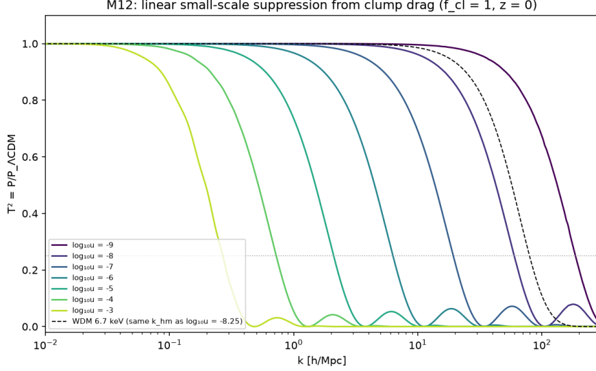
Figure 5: Linear matter transfer function T^2 = P/P_{\Lambda\text{CDM}} at z = 0 for couplings from u = 10^{-9} to 10^{-3} , with all dark matter in clumps. The dashed line is a thermal-relic warm dark matter model with the same half-mode wavenumber as the u = 10^{-8.25} clump model. The clump models show the damped oscillations characteristic of a species that was coupled to an oscillating fluid.
