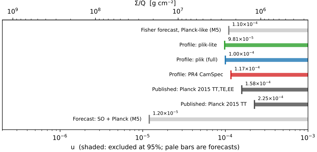
Figure 2: Summary of the 95% upper limits on u , with the equivalent minimum clump surface density on the upper axis. Shaded bars mark the excluded region. The pale bars are forecasts: the Planck-like Fisher forecast made before the data were used, and the forecast for Simons Observatory combined with Planck, which would improve the limit by nearly an order of magnitude.
