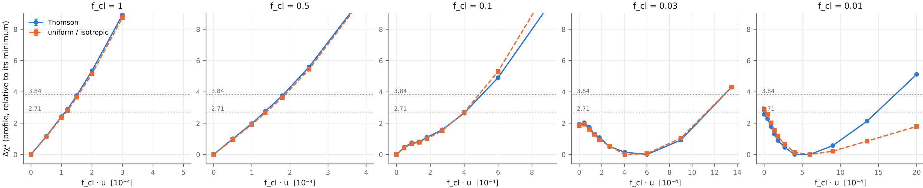
Fixed-fraction profiles in the clump coupling, PR4 CamSpec + 2018 low- \ell
