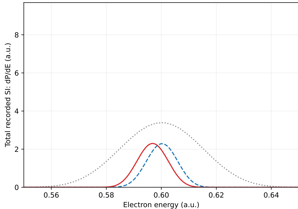
Later-ionization band near 0.6 a.u.
