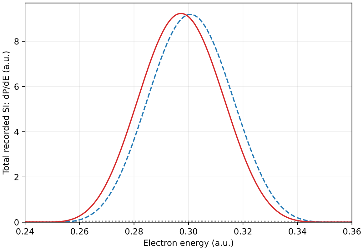
Original-electron band near 0.3 a.u.
