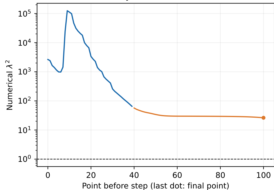
Higher-energy unitarity still fails
