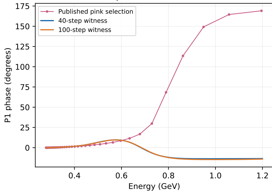
Published phases remain unmatched
