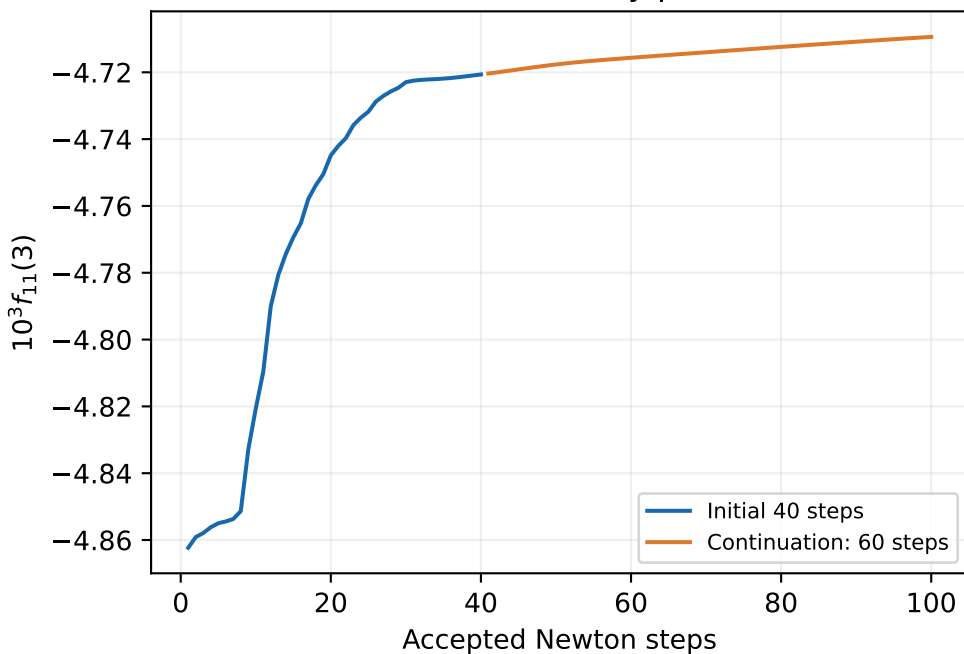
Published phases remain unmatched
