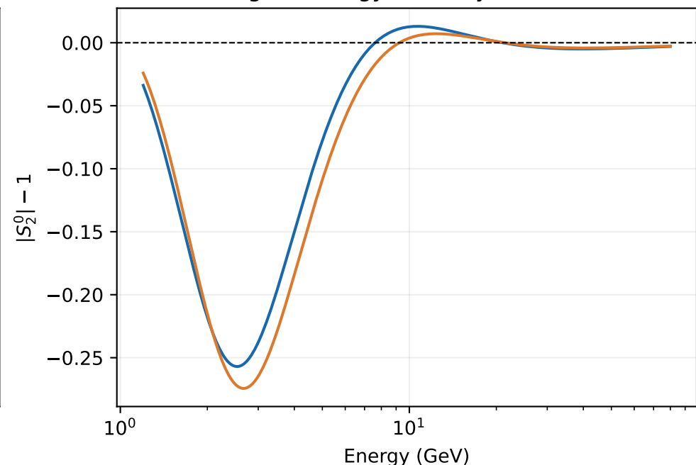
Higher-energy unitarity still fails
