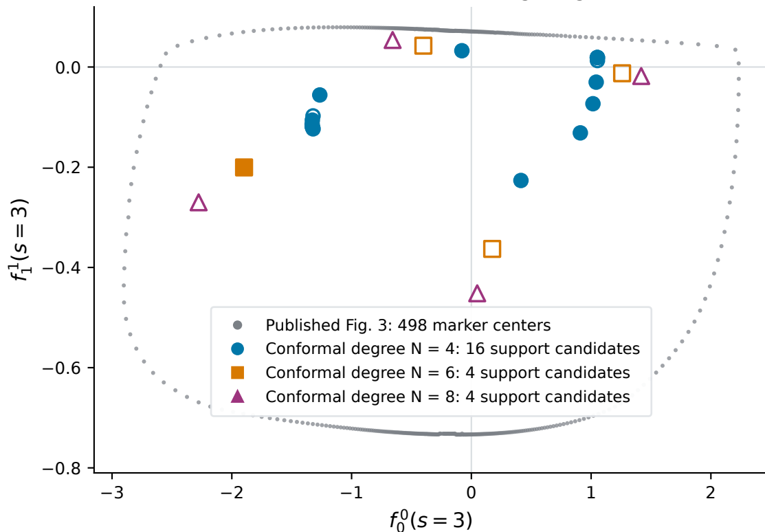
A Finite-truncation scattering diagnostics
