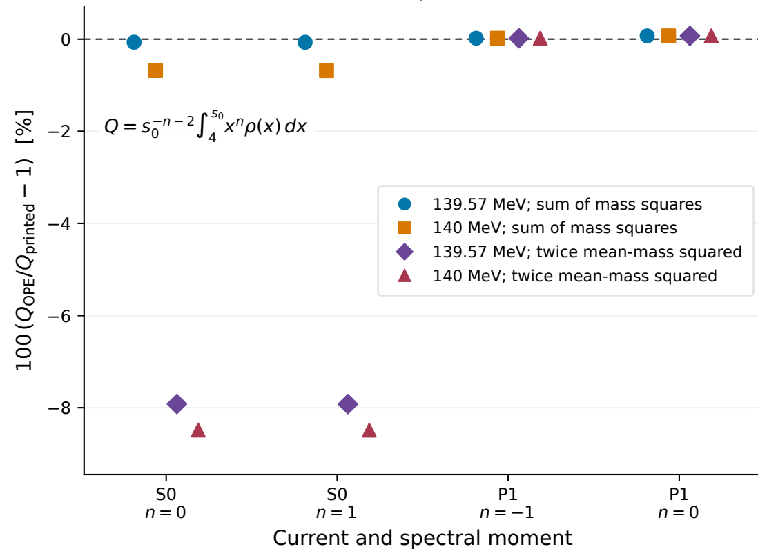
B Normalization and quark-mass conventions
