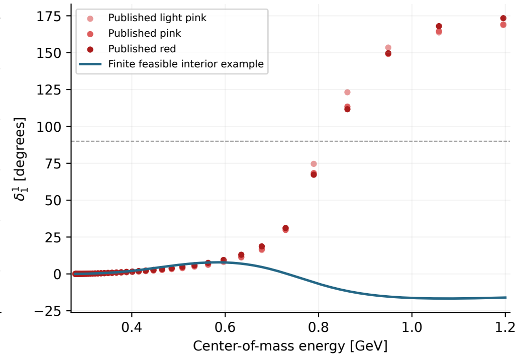
D. Exact statement for the gauge example
