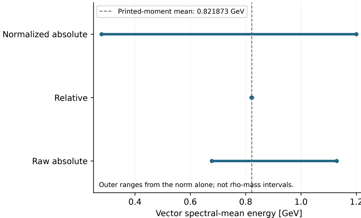
C. Information retained by the moment norm
