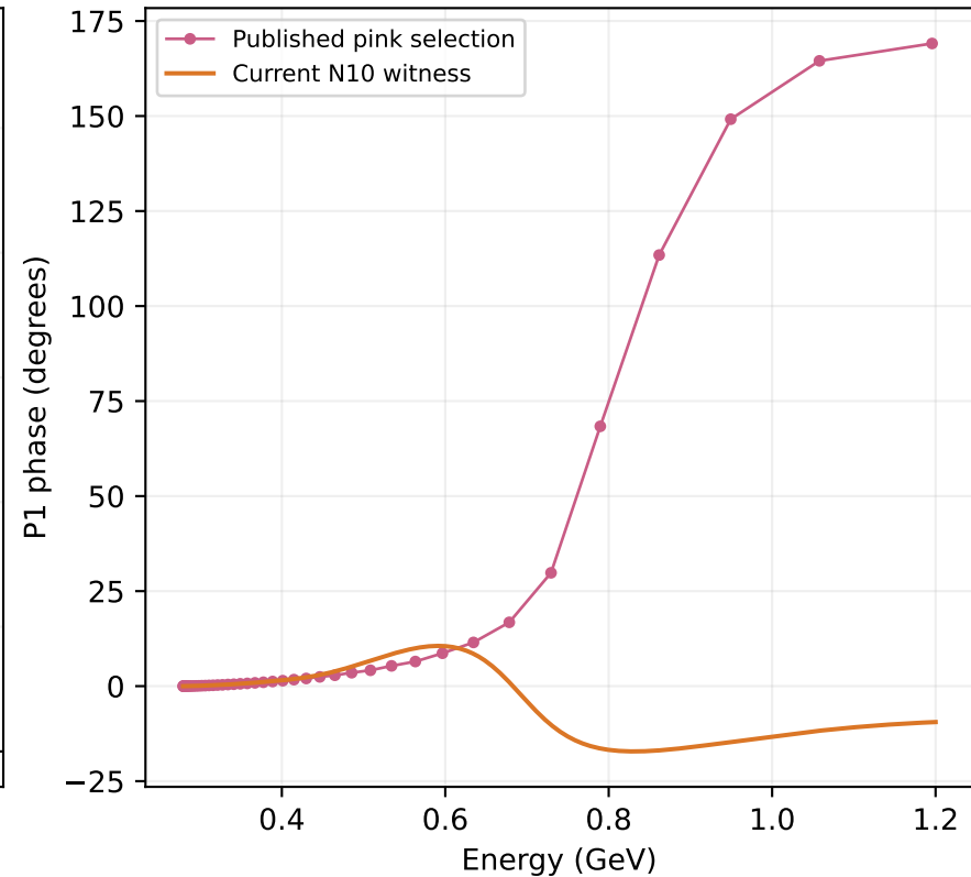
Published phase curve not reproduced
