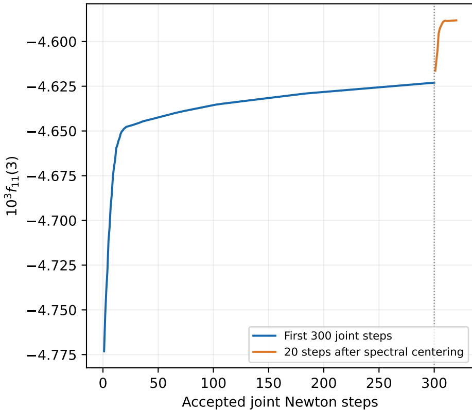
Strict finite feasibility preserved
