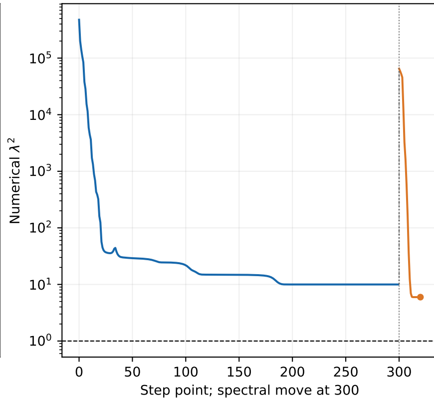
Full centrality still unresolved
