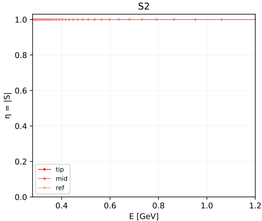
The same three amplitudes: native inelasticities
