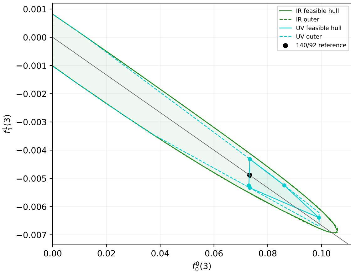
Fig.8: fixed chiral setting, with current/QCD constraints
