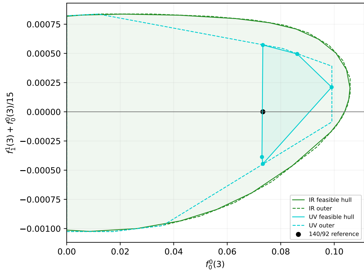
Fig.8: fixed chiral setting, with current/QCD constraints
