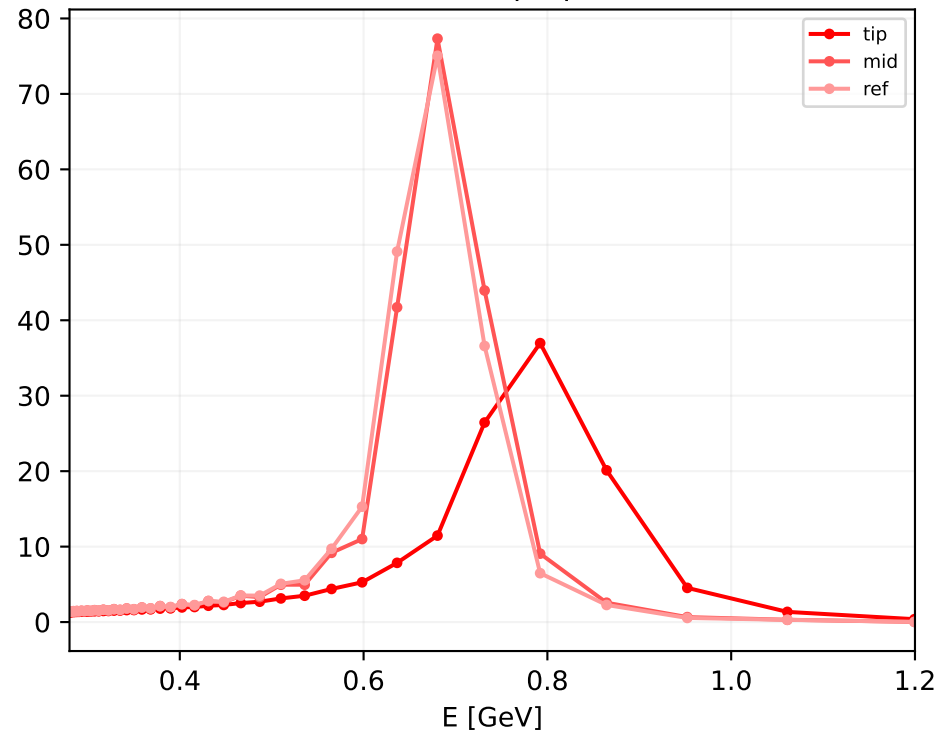
Fixed amplitudes: native peaks; no pole fit Vector |F1|^2
