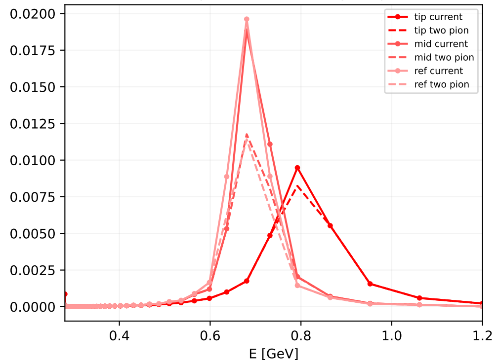
Vector spectrum and two-pion part
