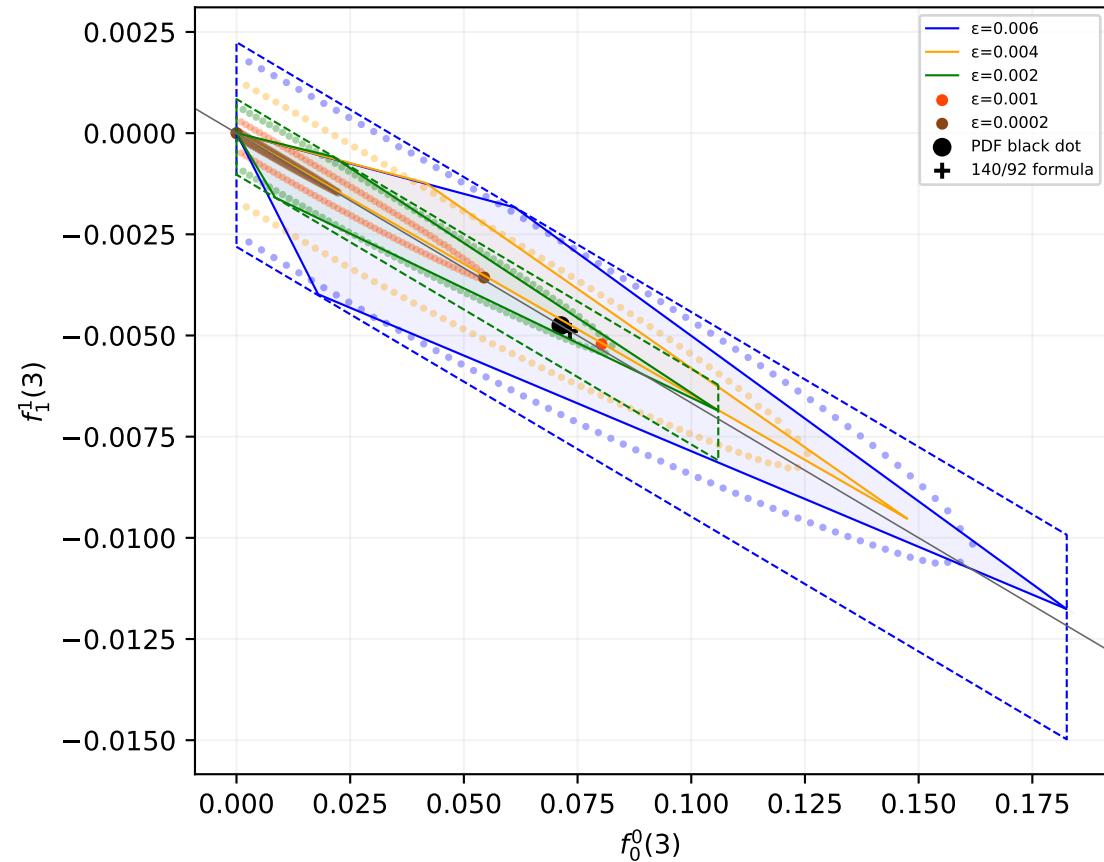
Fig.4: chiral supports
