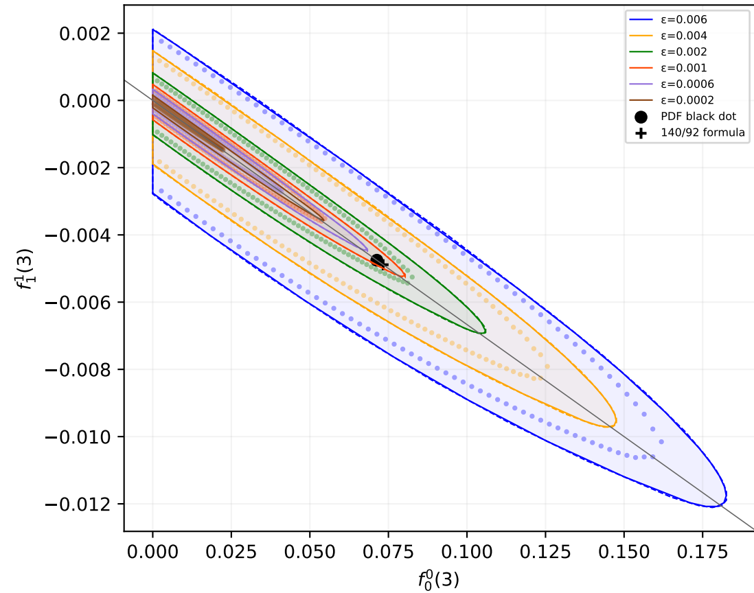
Fig.4: chiral supports
