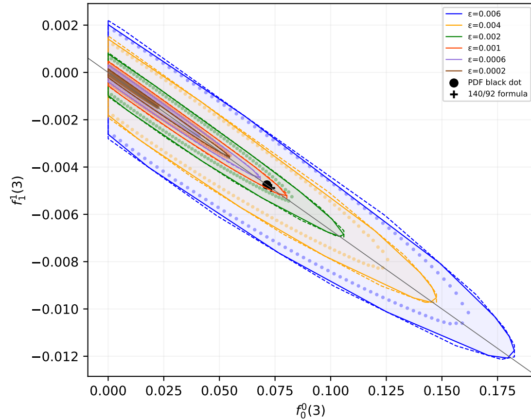
Fig.4: chiral supports
