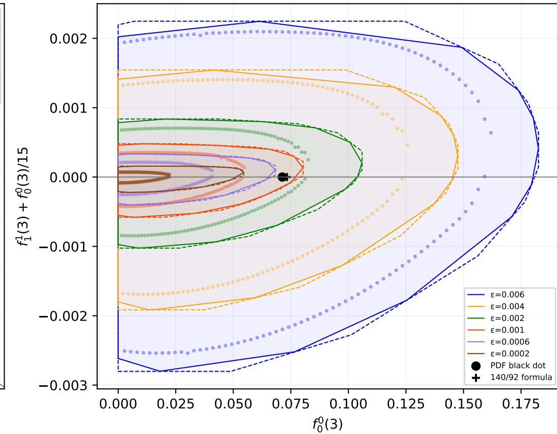
Chiral widths: y+x/15
