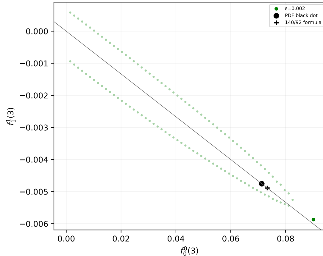
Fig.4: chiral supports
